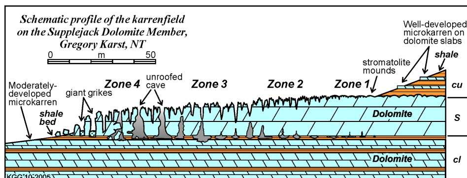
Figure 12: Schematic profile of a karrenfield in the Gregory Karst Region, Northern Territory. cu , upper Skull Creek Formation; S , Supplejack Dolomite member; cl , lower Skull Creek Formation. Zone 1, Incipient karren; Zone 2, moderately-developed grikes and spitzkarren; Zone 3, deep grikes and large spitzkarren; Zone 4, giant grikes, unroofed caves, sculptured pinnacles and stone city.
