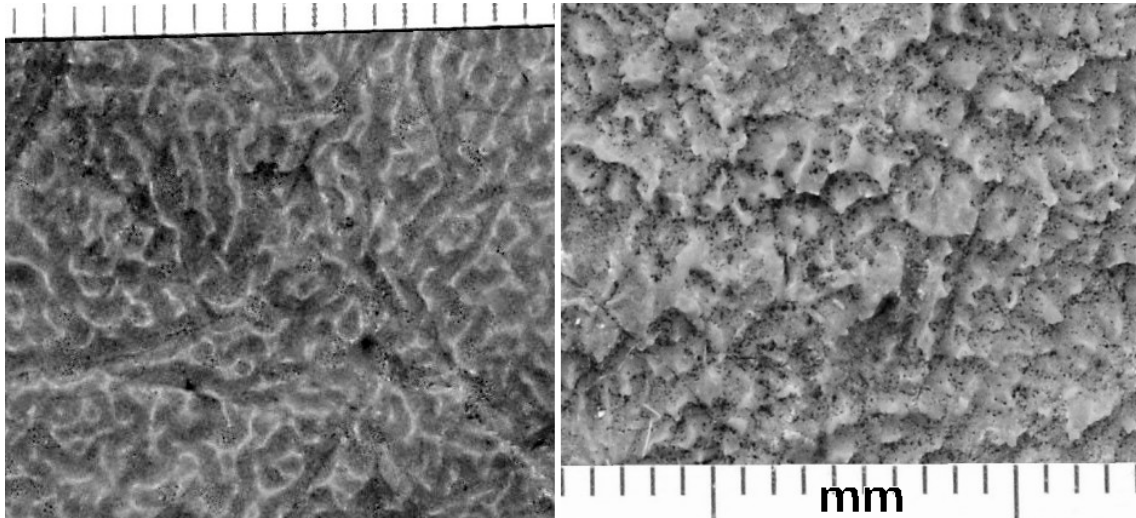
Figure 9: Microkarren on a pediment at Chillagoe. Left: network of small furrows and ridges; Right: rasp-like teeth. Scales in mm.
