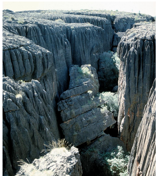
Figure 11: A giant grike, about 5 metres wide, with collapsed blocks and deep vertical wandkarren. Above Mimbi Cave, Kimberly region. Note the relatively undissected plateau in the background. Photo by J. Jennings.
