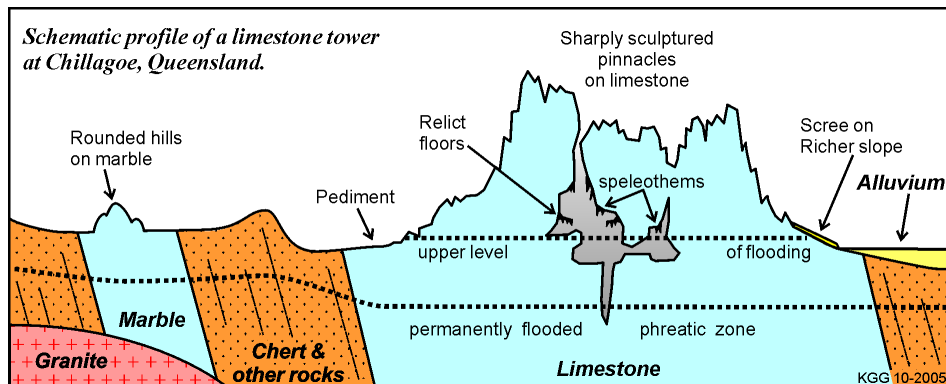
Figure 4: Schematic profile of a limestone tower at Chillagoe, Queensland.
